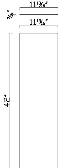
Wall End Panel 12*42*3/16
