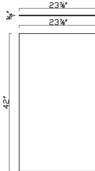
Skin Panel 24*42*1/4"
