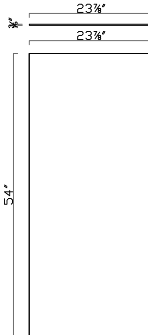
Skin Panel 24*54*1/4"
