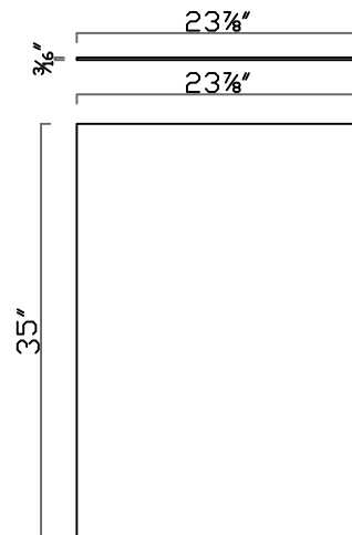
End Panel 24*35*3/16
