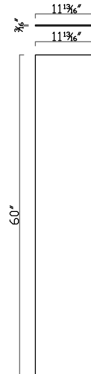
Skin Panel 12*60*1/4"
